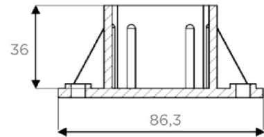
Instaling clamps for panels MEP.1 and MEP.2
